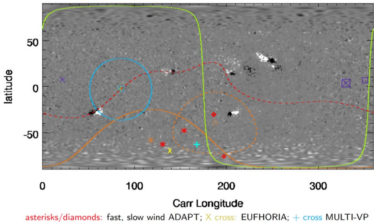
Figure 2. Benchmarking the connectivity estimates performed by the MADAWG team using past data. The figure shows a SDO/HMI magnetogram with magnetic footprints of fieldlines connected with the expected Solar Orbiter position using a variety of methods and models (orange, red, yellow and cyan symbols). The blue square indicates the position of the spacecraft, and the green line its visible limbs. The red line indicates the heliospheric current sheet. The violet symbols indicate Parker Solar Probe position and footprints at the same instant.
