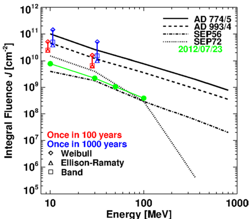
Figure 4. The 100-year and 1000-year data pointed derived from the cumulative distributions are superposed on the spectra of the AD774 and AD993 particle events obtained by Mekhaldi et al., 2015. Estimates of 100-year and 1000-year event sizes from Weibull, Ellison-Ramaty and Band functions are shown using different symbols. The spectra of the 1956 February 23 (SEP56) and 1972 August 4 (SEP72) solar proton events are also shown from Mekhaldi et al., 2015, who used the re-evaluated spectra from Webber et al., 2007. Also shown is the spectrum of the 2012 July 23 extreme event from Gopalswamy et al., 2016 (from Gopalswamy 2017).
