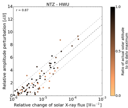
Figure 1: Relative VLF amplitude perturbations over the relative X-ray flux change of solar flares derived from the VLF path between HWU (France: 20.9 kHz) to Neustrelitz.
