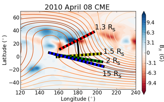
Figure 1: ForeCAT results for the 2010 April 8 CME, which match the observed trajectory. The color contours show the magnetic field at the solar surface. The line contours show the magnetic field farther out, with the darkest lines indicating the location of the Heliospheric Current Sheet (HCS). The CME is initiated parallel to the polarity inversion line of an active region. The CME deflects south along the HCS and the rotation brings the CME orientation more parallel to that of the nearby HCS.
