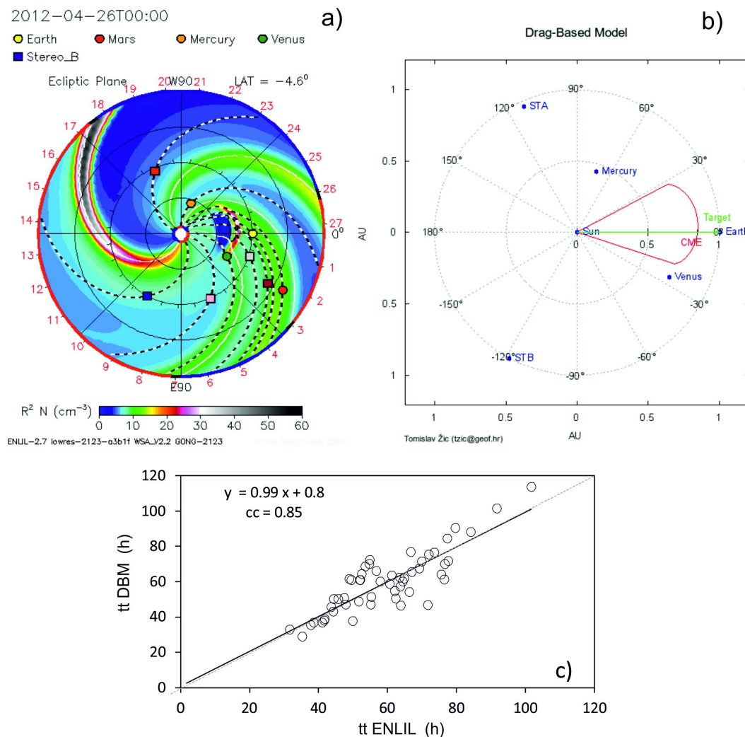
Figure 2. Comparison of numerical ENLIL code and analytic Drag-Based Model (DBM).
