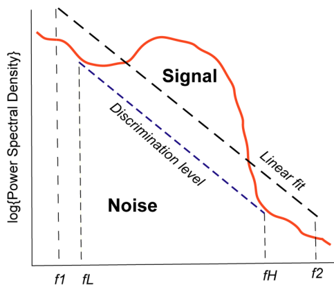
Figure 1. Schematic plot of the technique for the discrimination of signal and noise from the power spectral density of ULF variations.
