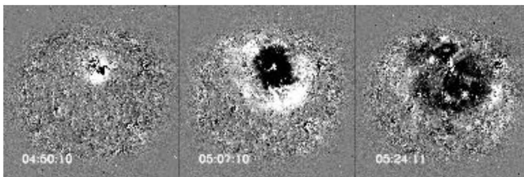
Figure 1. An “EIT wave” event observed on 12-May-1997 by the SOHO/EIT instrument. These running difference images (wherein a following image is subtracted from a leading image) are used to highlight the moving pulse and make it easier to identify in single images.
