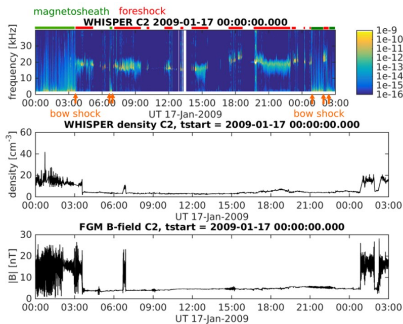
Figure 1: Example of CLUSTER 2 measurements in the vicinity of the terrestrial bow shock on 17 January 2009. (Top) Time-frequency spectrogram of one electric component observed by the WHISPER instrument. Orange arrows show bow shock crossings. Magnetosheath and foreshock visits are labeled by green and red bars, respectively. (Middle) The local electron density obtained from the WHISPER measurements. (Bottom) The total magnetic field calculated from the Fluxgate magnetometer.
