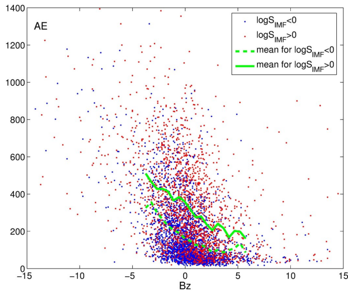
Figure 3. Comparison of the auroral response, as characterized by hourly AE index, with the strength of the SW driver, determined by the IMF Bz component, for the calm ( \log S_{IMF} < 0 , blue dots) and turbulent ( \log S_{IMF} > 0 , red dots) IMF for the period 1994-1995 from Romanova et al . , 2008.
