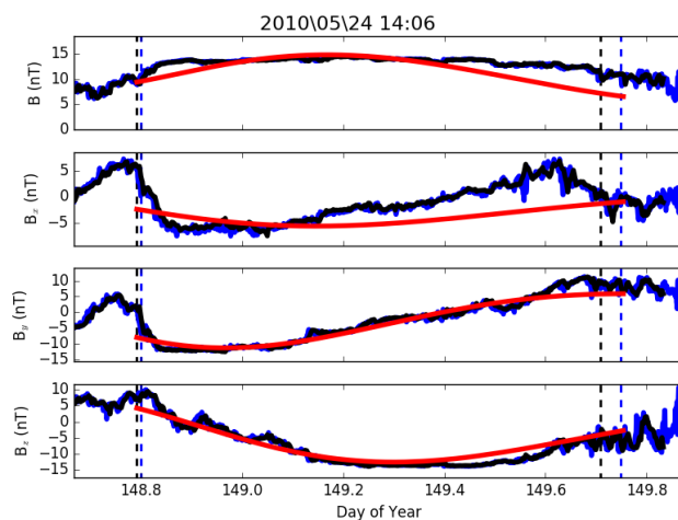
Figure 2: FIDO results for the 2010 May 24 CME. The black and blue lines correspond respectively to the ACE and Wind data and the red line shows the FIDO simulation.
