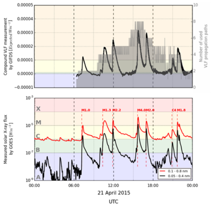
Figure 2: Compound VLF measurement and the corresponding solar X-ray flux measured by GOES.
