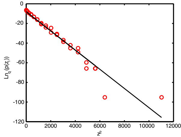
Fig. 2. Linear correlation between \ln_q[p(z_i)] and z_i^2 , where q_{\text{stat}} = 1.32 \pm 0.06 . The linear CC. is 0.9383.
