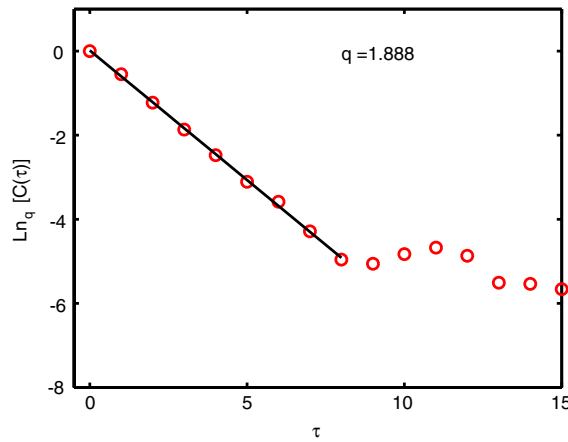
Fig. 4. \ln_q of the self-correlation coefficient C(\tau) vs. time delay \tau (in days). We obtain the best fit with q_{rel} = 1.888 . The linear CC is 0.99919.
