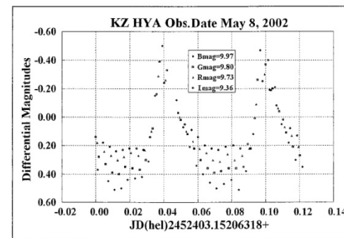
Figure 3. The observation of CCD photometry of the KZ Hya with BGR colors which were made during the night of May 8, 2002
